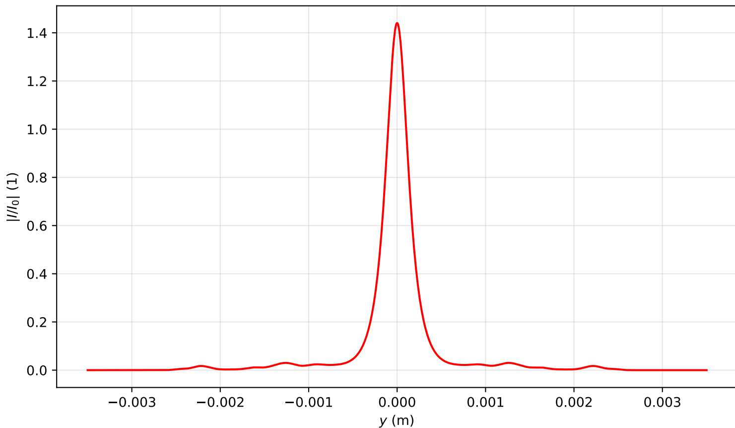
Intensity profile I(x=0, y, z=3.582)/I_0 , P_{in}=4.0P_{cr} , artificial time
